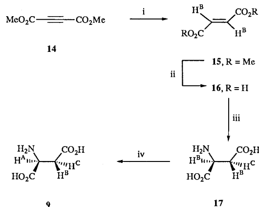
Scheme 3 Reagents and conditions: i, Ph 3 P, 2 H 2 O, THF; ii, 12% NaOH, 41% over 2 steps; iii, β-methylaspartase, NH 3 , K + , Mg 2+ , water, 60%; iv, AAT, PLP, water, 78%
